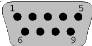
Figure 5 – SGI 9–Pin Connector
