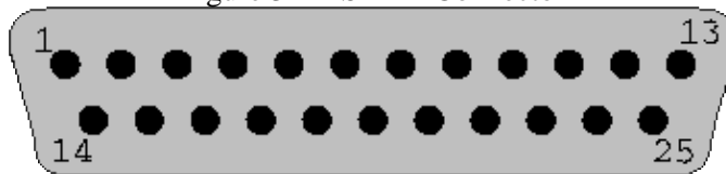
Figure 3 – RS-422 Connector
